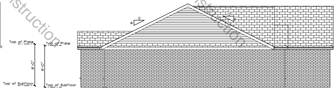
LEFT ELEVATION
